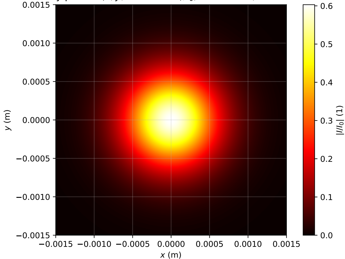
Intensity profile I(x, y, z = 2.468m)/I_0 , P_{in}=0.4P_{cr} , artificial time
